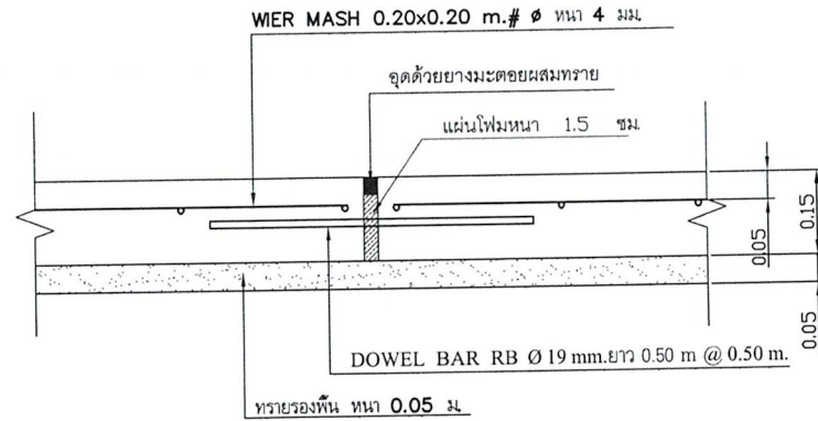
EXPANSION JOINT
