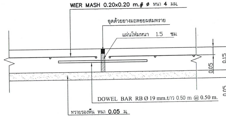
EXPANSION JOINT
