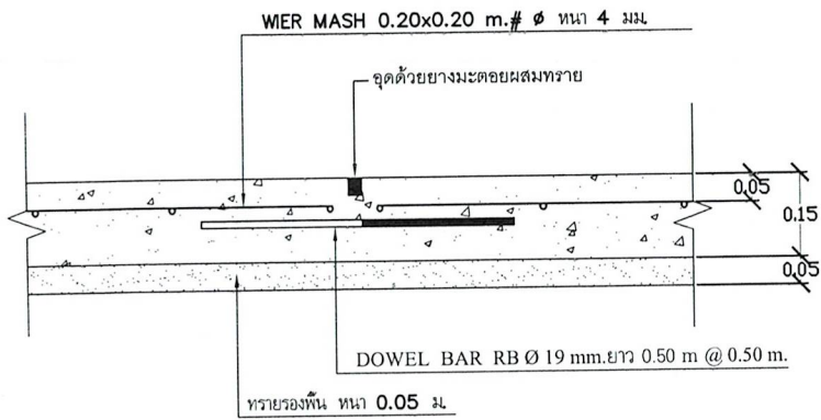
CONTRACTION JOINT
