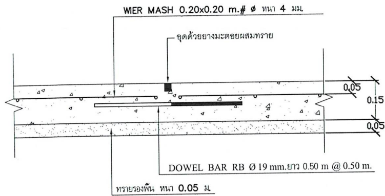
CONTRACTION JOINT
